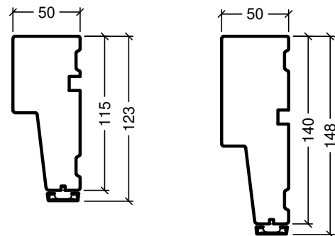
Frame variants outward opening doors
