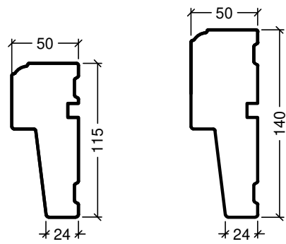
Frame variants outward opening doors
