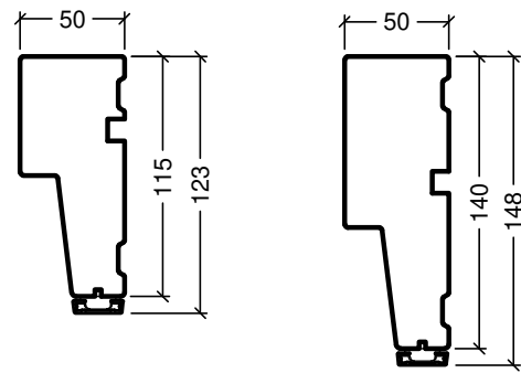
Frame variants outward opening doors
